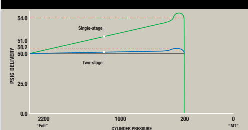
PRESSURE REGULATION
